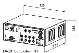
D620i Controller IP43
