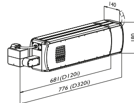
Laser head D120i and D320i (i-Tech i0)
