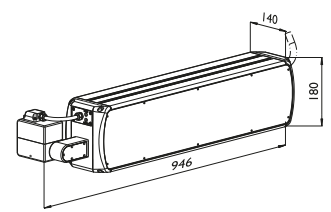
Laser head D620i IP65 (i-Tech IP65)
