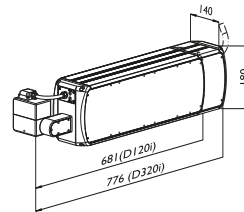
Laser head D120i and D320i IP65 (i-Tech IP65)
